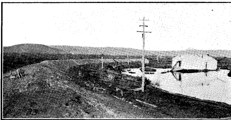
ELECTRIC SUCTION DREDGE FORMING EMBANKMENT.
