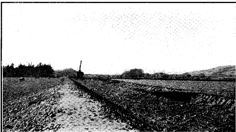
DRAG-LINE EXCAVATOR AT WORK FORMING LEVEE. TAIERI RIVER FLOOD PROTECTION.
