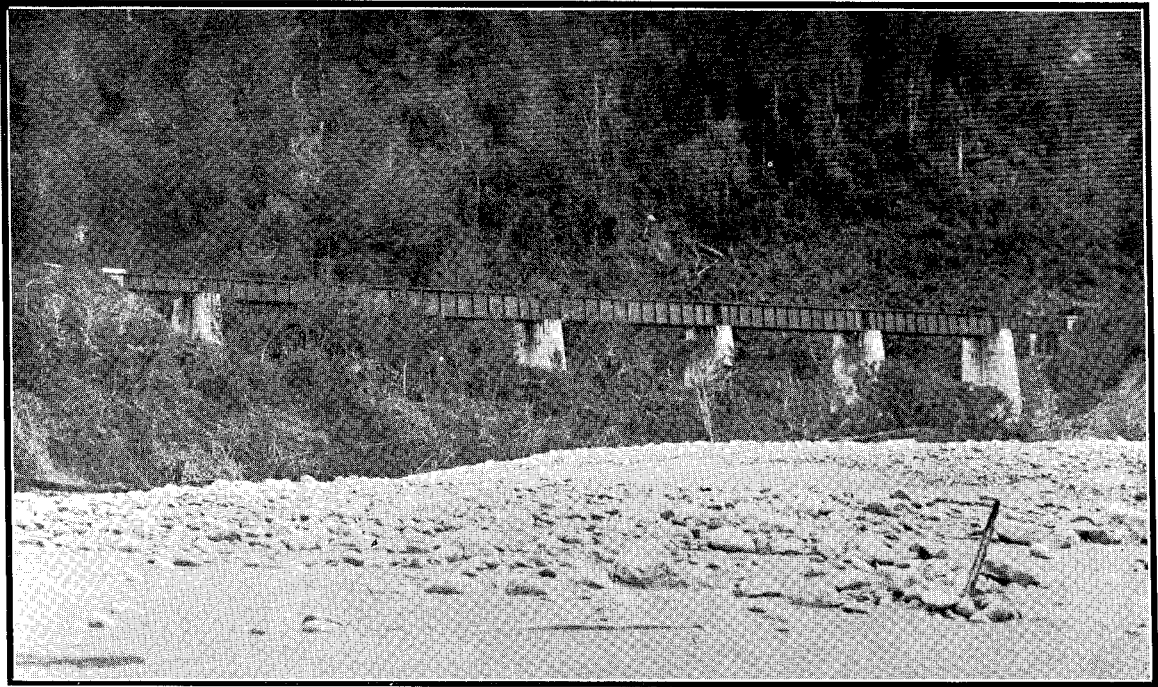
LITTLE CASCADE CREEK BRIDGE. Four 50 ft., two 30 ft., and one 20 ft. spans. WESTPORT - INANGAHUA RAILWAY.
