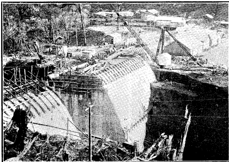
MANGAHAO NO. 3 DAM UNDER CONSTRUCTION.
