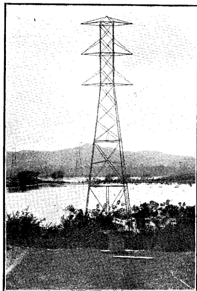
TRANSMISSION - LINE TOWERS ON MAIN AUCKLAND-ARAPUNI LINE.
