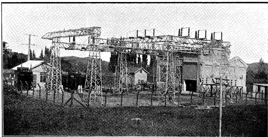
NAPIER SUBSTATION.
