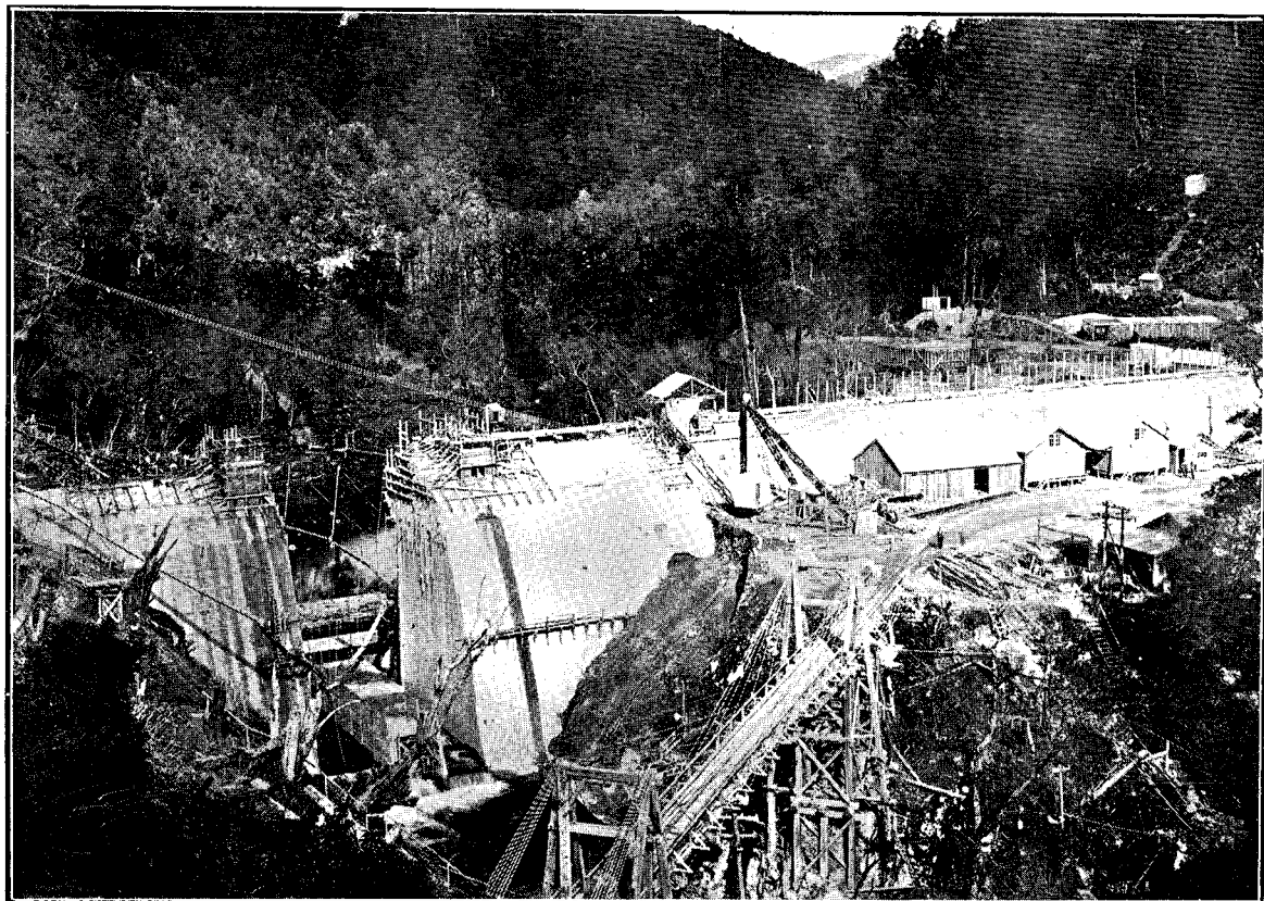
NO. 3 DAM UNDER CONSTRUCTION.
