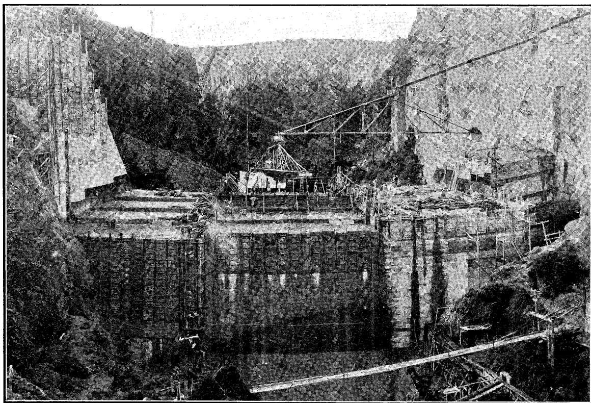
ARAPUNI DAM : POSITION OF WORK AT 3RD AUGUST, 1927.
