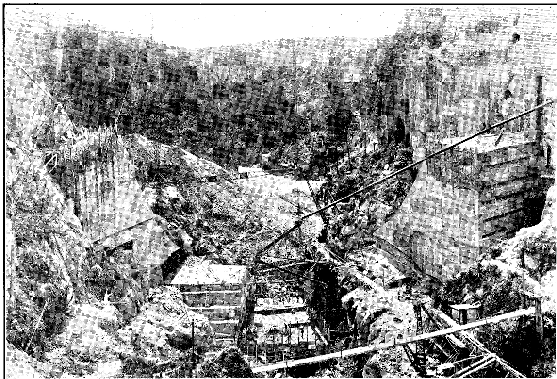
ARAPUNI DAM : COMMENCING CONCRETE IN BOTTOM.
