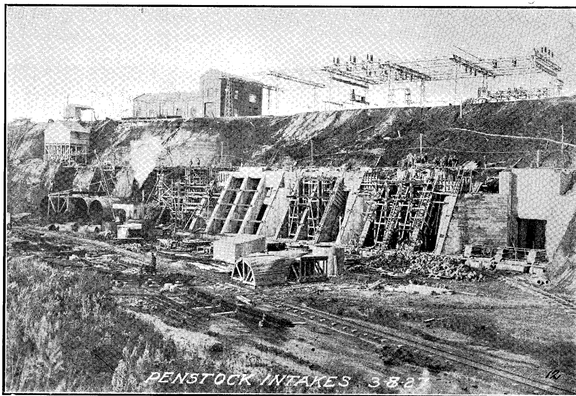
PENSTOCK INTAKES.
