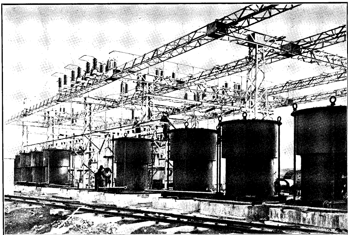
OUTDOOR TRANSFORMER AND SWITCHING-STATION.
