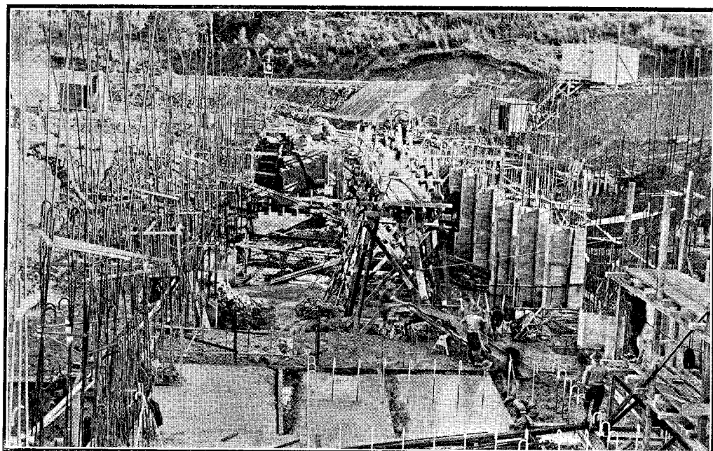
POWER-HOUSE FOUNDATIONS.
