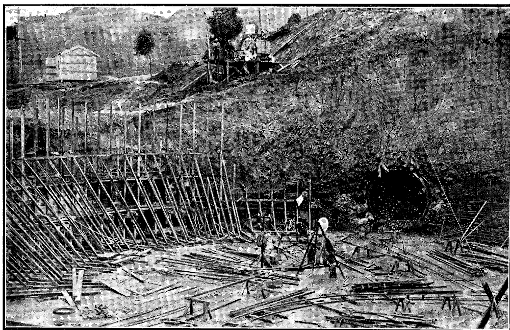
PART OF SURGE-CHAMBER AND TUNNEL-OUTLET. WAIKAREMOANA HYDRO-ELECTRIC SCHEME.
