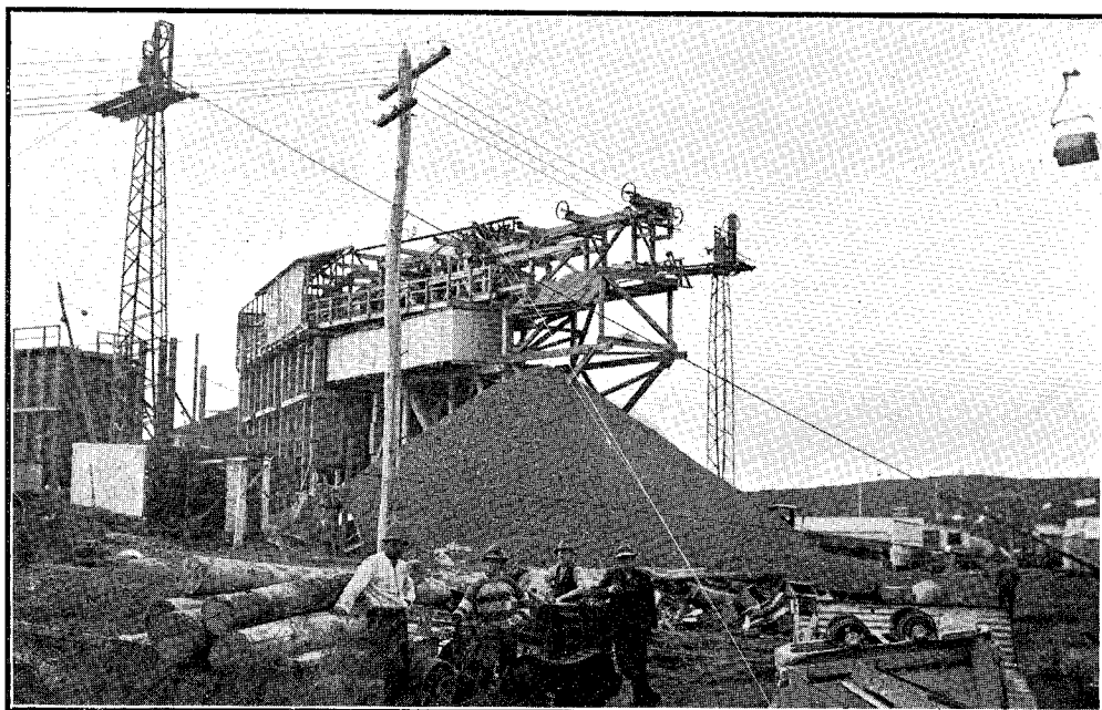
ROPEWAY TERMINAL, SHINGLE-BINS, ETC. ARAPUNI HYDRO-ELECTRIC SCHEME.
