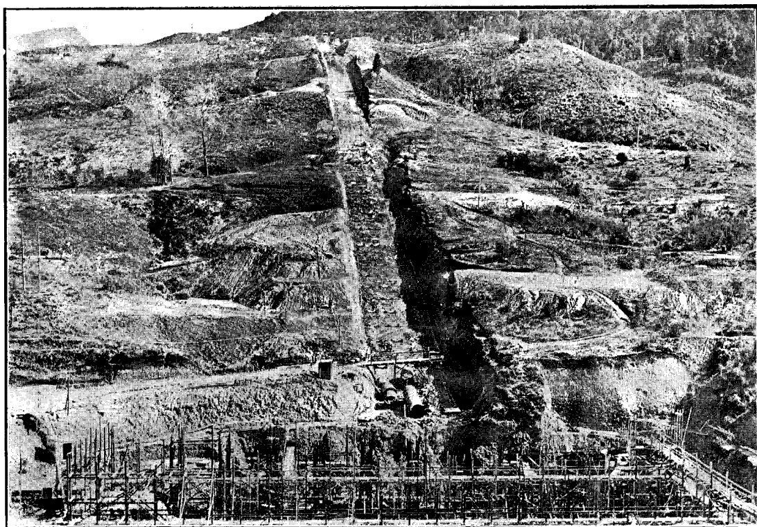
PIPE-LINE EXCAVATION FROM POWER-HOUSE.
