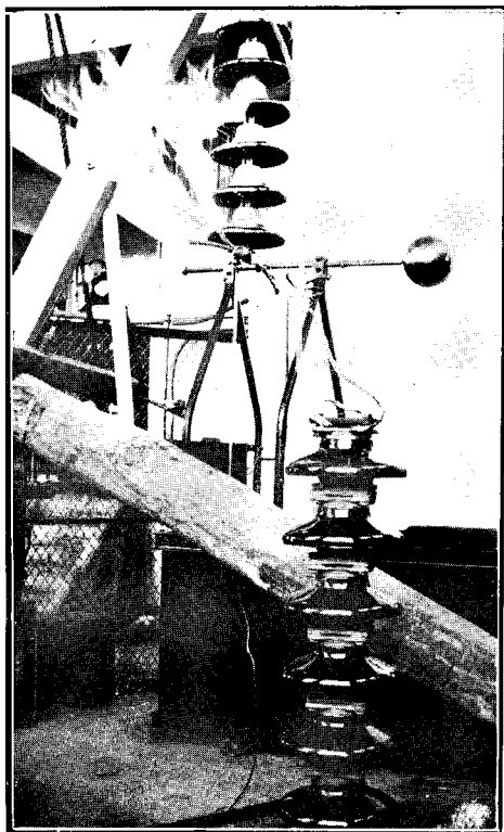
TESTING FLASH-OVER CLEARANCES ON INSULATOR STRINGS.
