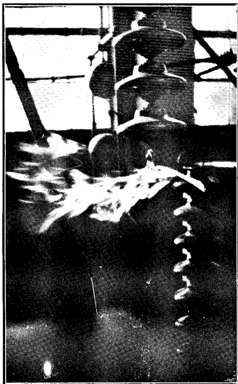
TESTING FLASH-OVER CLEARANCES ON INSULATOR STRINGS.
