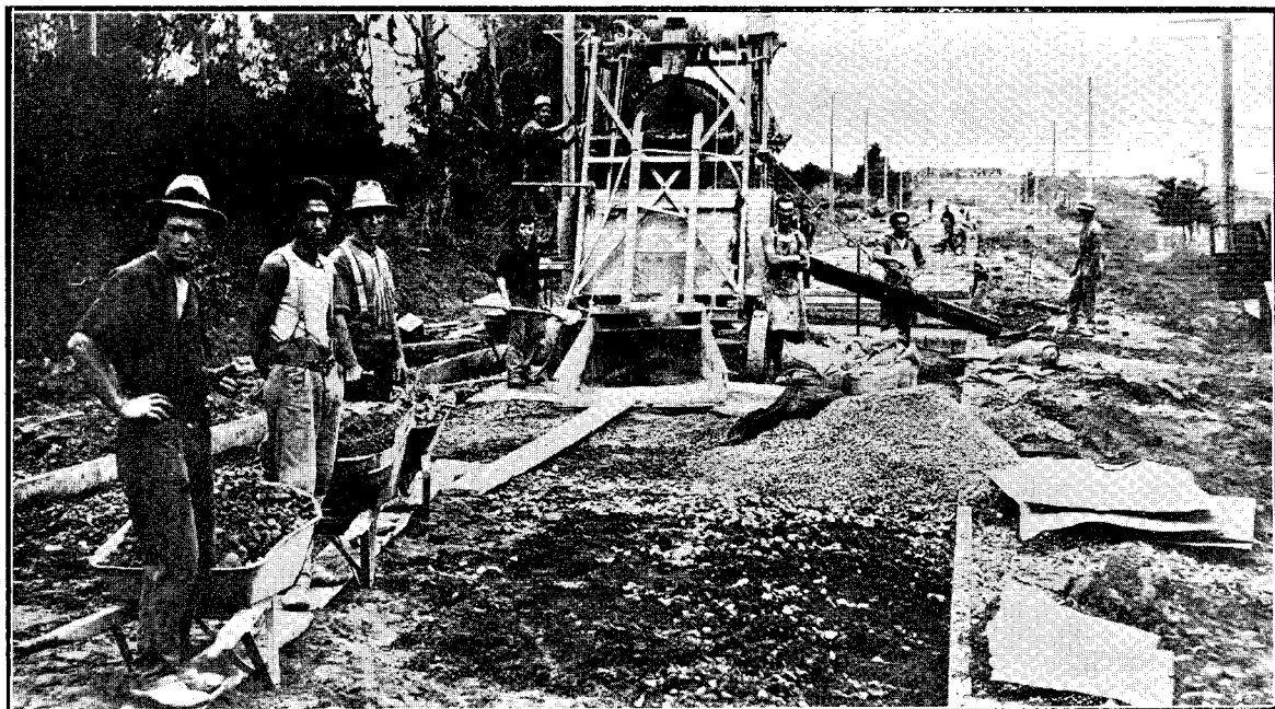
GREAT SOUTH ROAD, MANUREWA TOWN DISTRICT. Concrete paving in progress.
