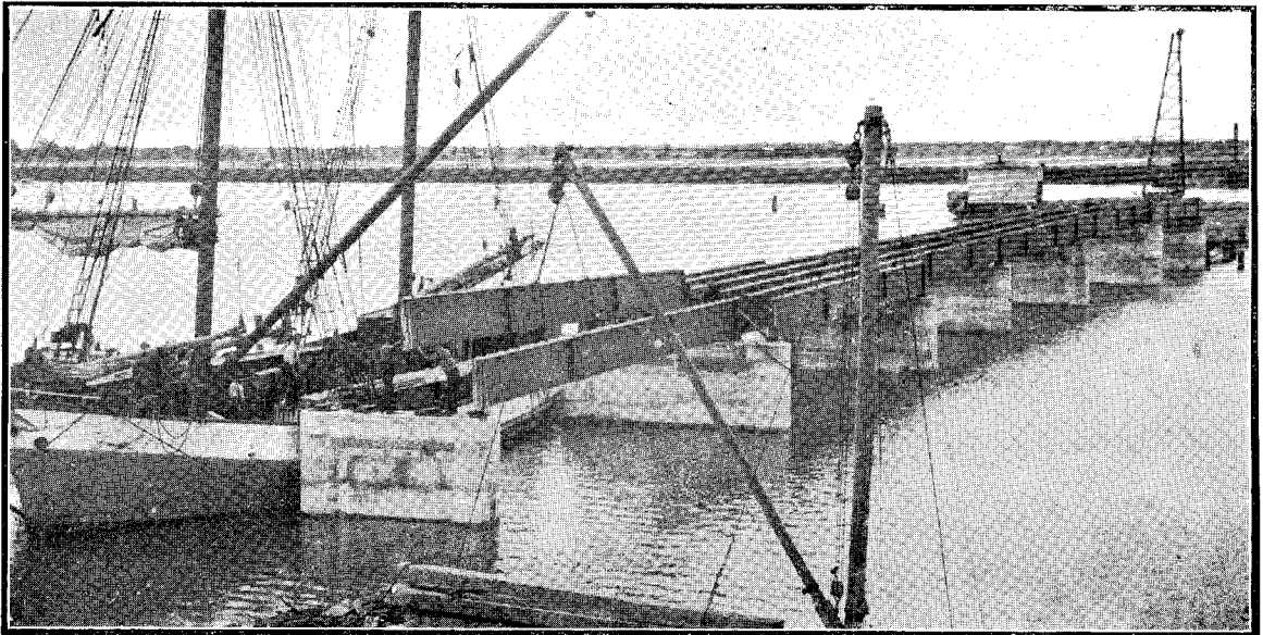
POKENO - WAIHI JUNCTION TO COROMANDEL MAIN HIGHWAY. Waihou River Bridge at Kopu : Unloading girders from scow "Rangi," and placing in position.
