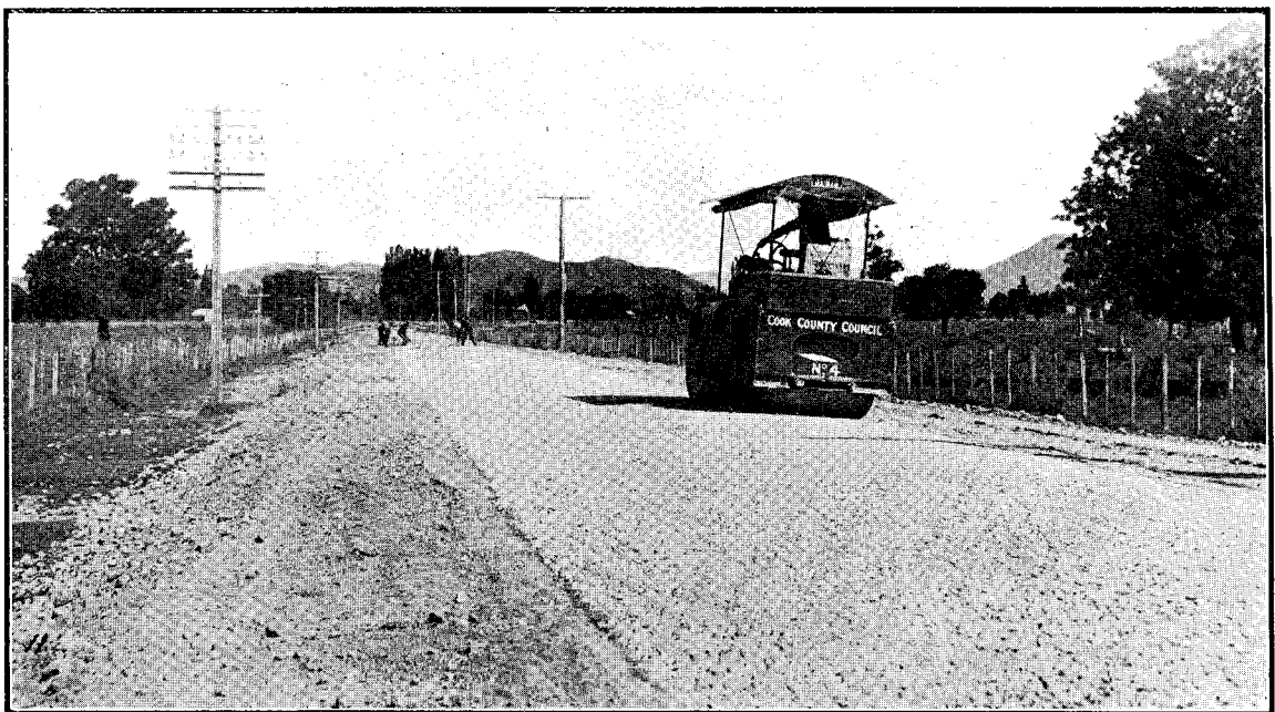
GISBORNE-NAPIER (VIA WAIROA) MAIN HIGHWAY, COOK COUNTY SECTION. Bituminous penetration surfacing ; rolling before spraying.
