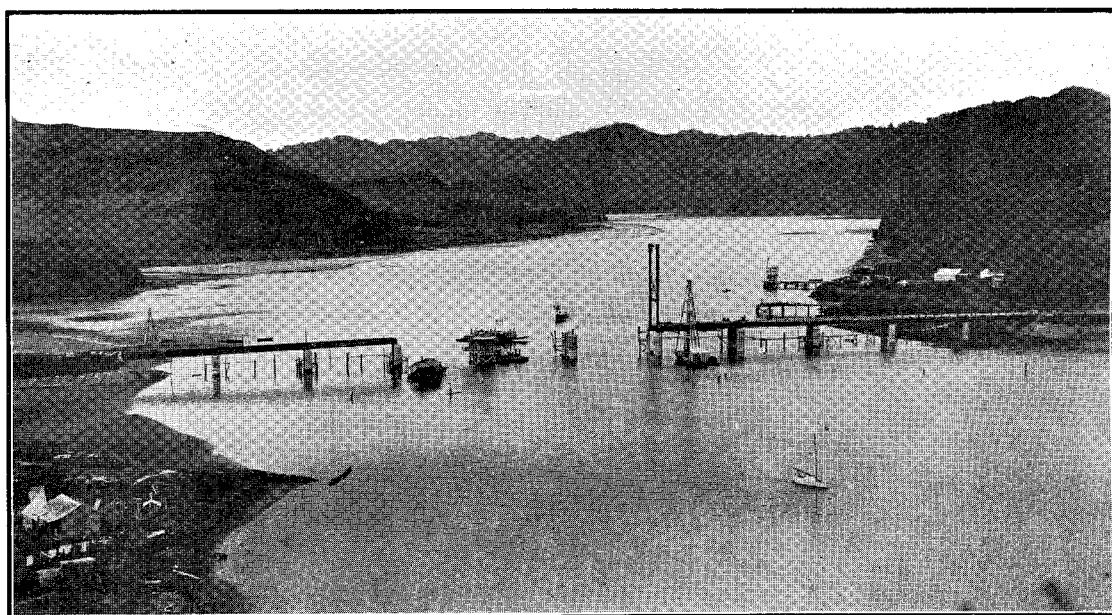
AUCKLAND-WELLINGTON (VIA TARANAKI) MAIN HIGHWAY. Mokau Bridge, under construction.
