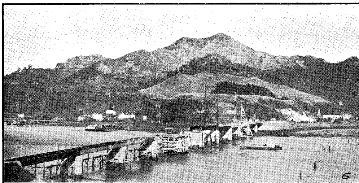
AUCKLAND-WELLINGTON (VIA TARANAKI) MAIN HIGHWAY. Mokau Bridge, under construction.
