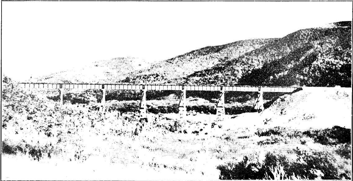
WALNUT RIVER BRIDGE. Seven 35 ft. steel plate girder spans.
