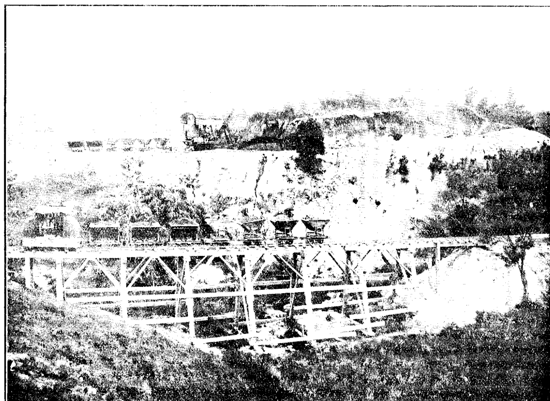
TOP LEFT OF CUTTING AT 34 M. NORTH AUCKLAND MAIN TRUNK RAILWAY. RANGIAHUA SECTION
