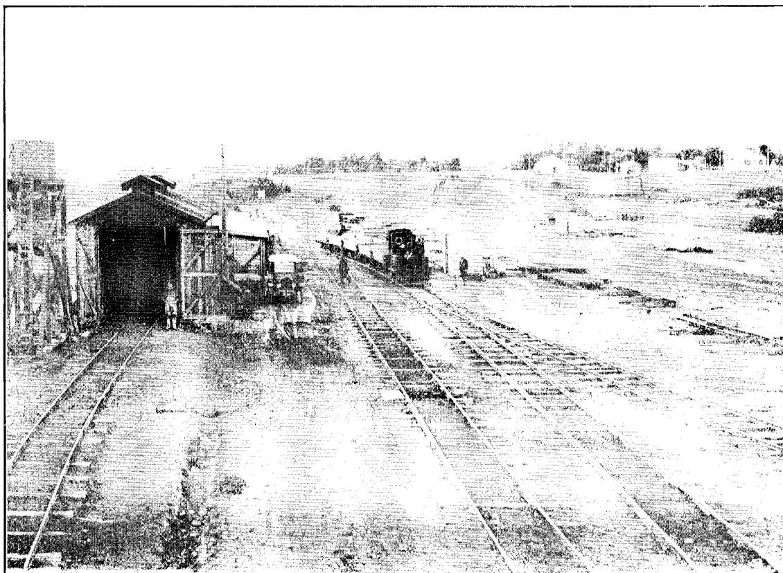
GENERAL VIEW OF EXCAVATION FOR GOODS YARD.
