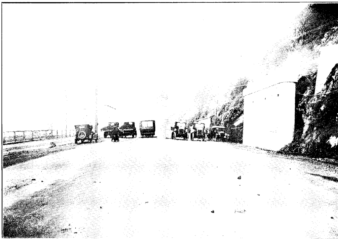
VIEW SHOWING PIERS FOR BRIDGE OVER HUTT ROAD AND RAILWAY. Note three lines of traffic through each span.
