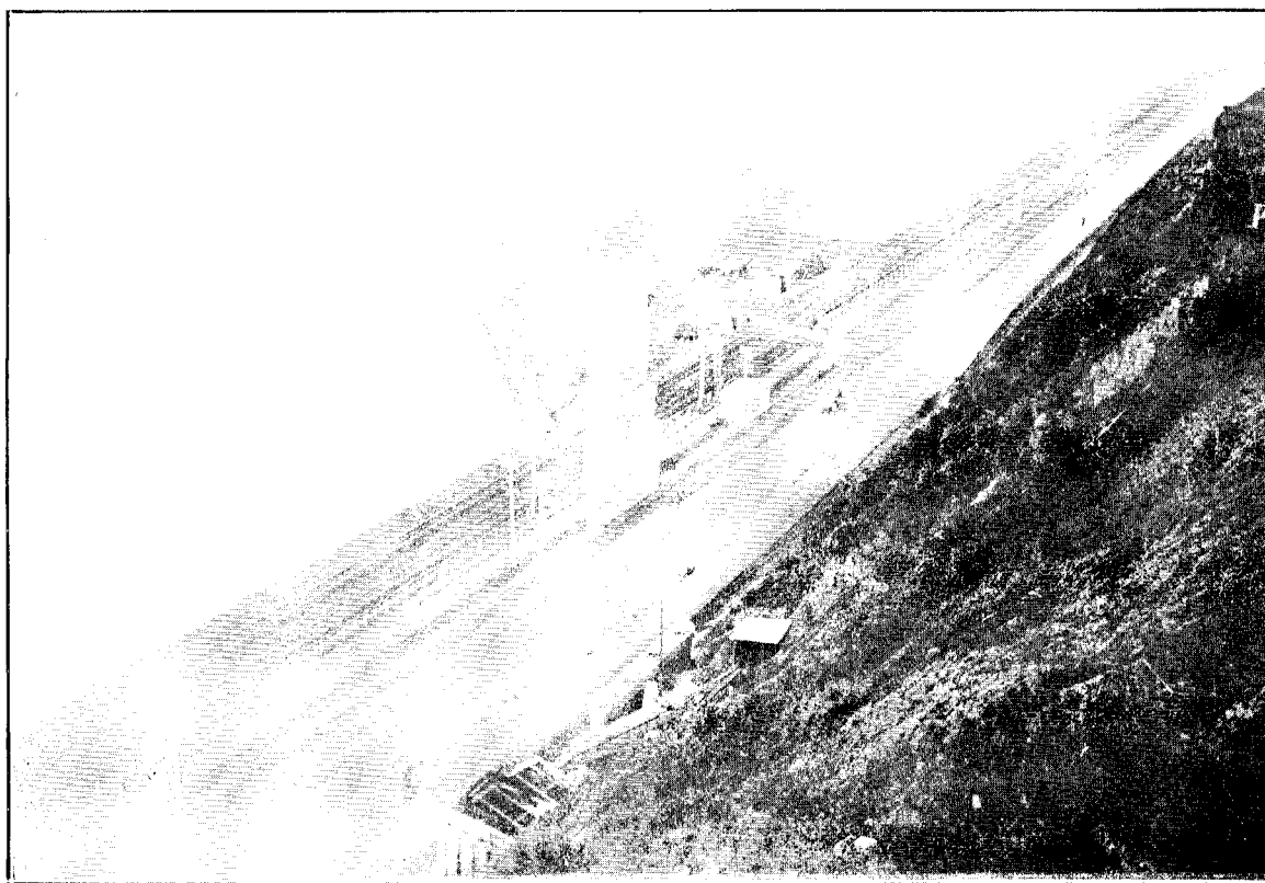
VIEW FROM ABOVE PORTAL OF NO. 1 TUNNEL. This view gives a good idea of the angle of skew of the crossing of road and railway, which is 60. WELLINGTON NEW PLYMOUTH RAILWAY. TAWA FLAT DEVIATION.
