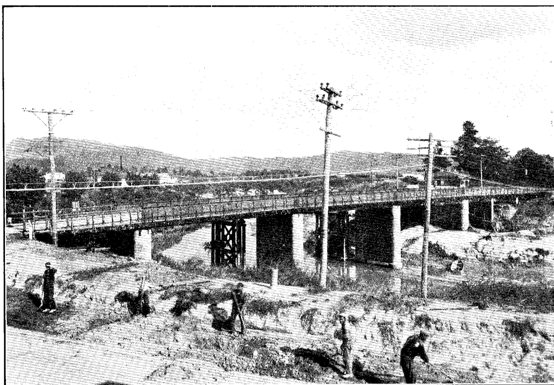
OHINEMURI RIVER ROAD-BRIDGE, PAEROA. Three 60 ft. through steel plate girder spans and four 30 ft. rolled steel joist spans. Concrete deck, 18 ft. roadway with footway on one side.
