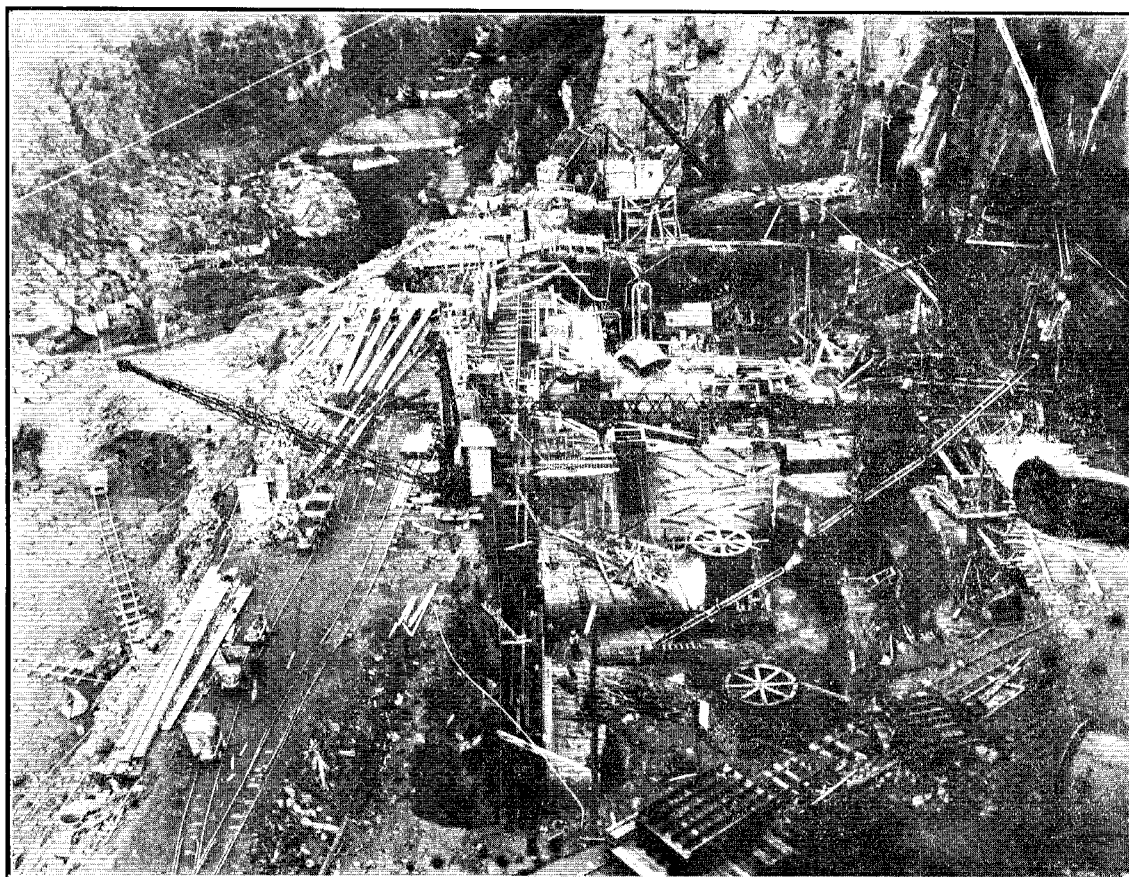
VIEW SHOWING EXCAVATION AT POWER-HOUSE SITE AND LOWER CONCRETE FOUNDATIONS IN PLACE.
