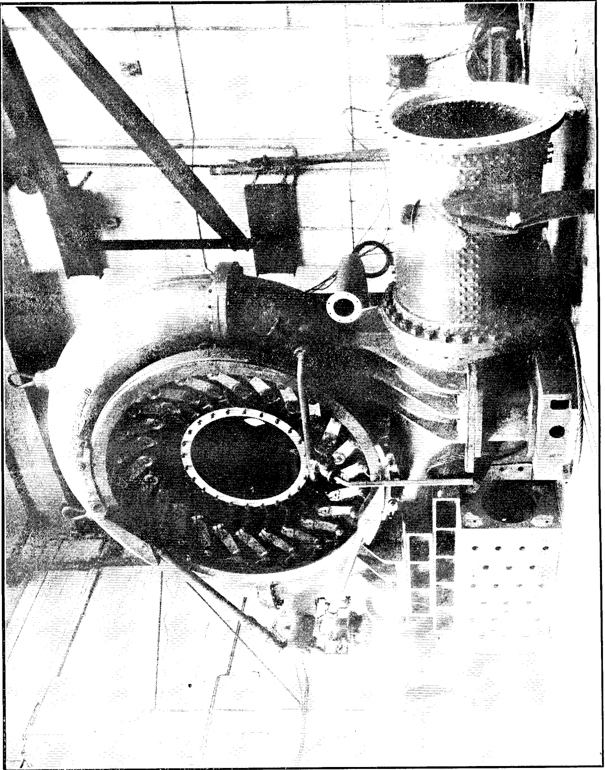
28,000 H.P. TURBINE ERECTED IN MAKER'S WORKSHOPS.
