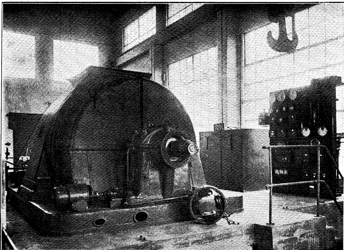
10,000 kv.a. SYNCHRONOUS CONDENSER, KHANDALLAH SUBSTATION.
