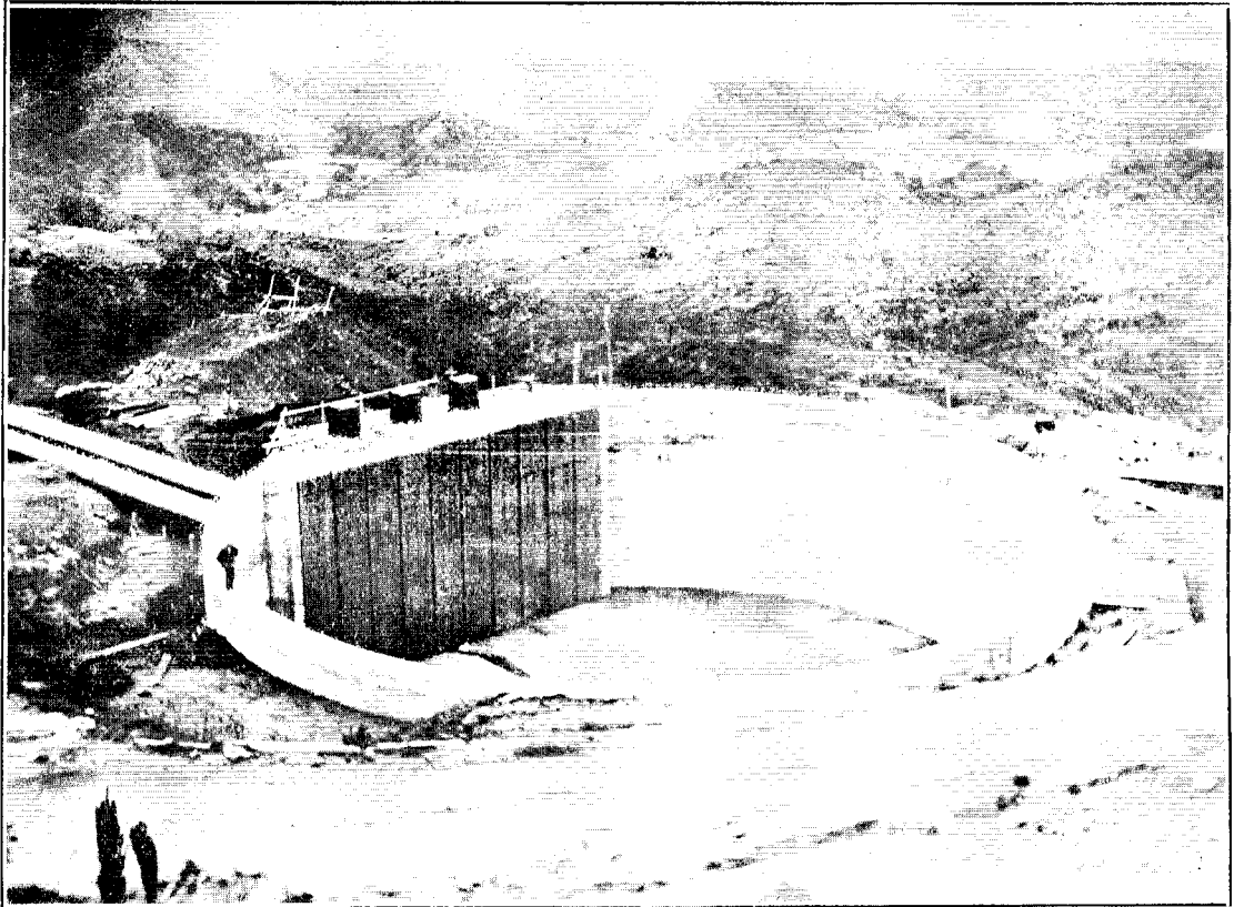
VIEW SHOWING SURGE CHAMBER WITH SCREENS IN POSITION.
