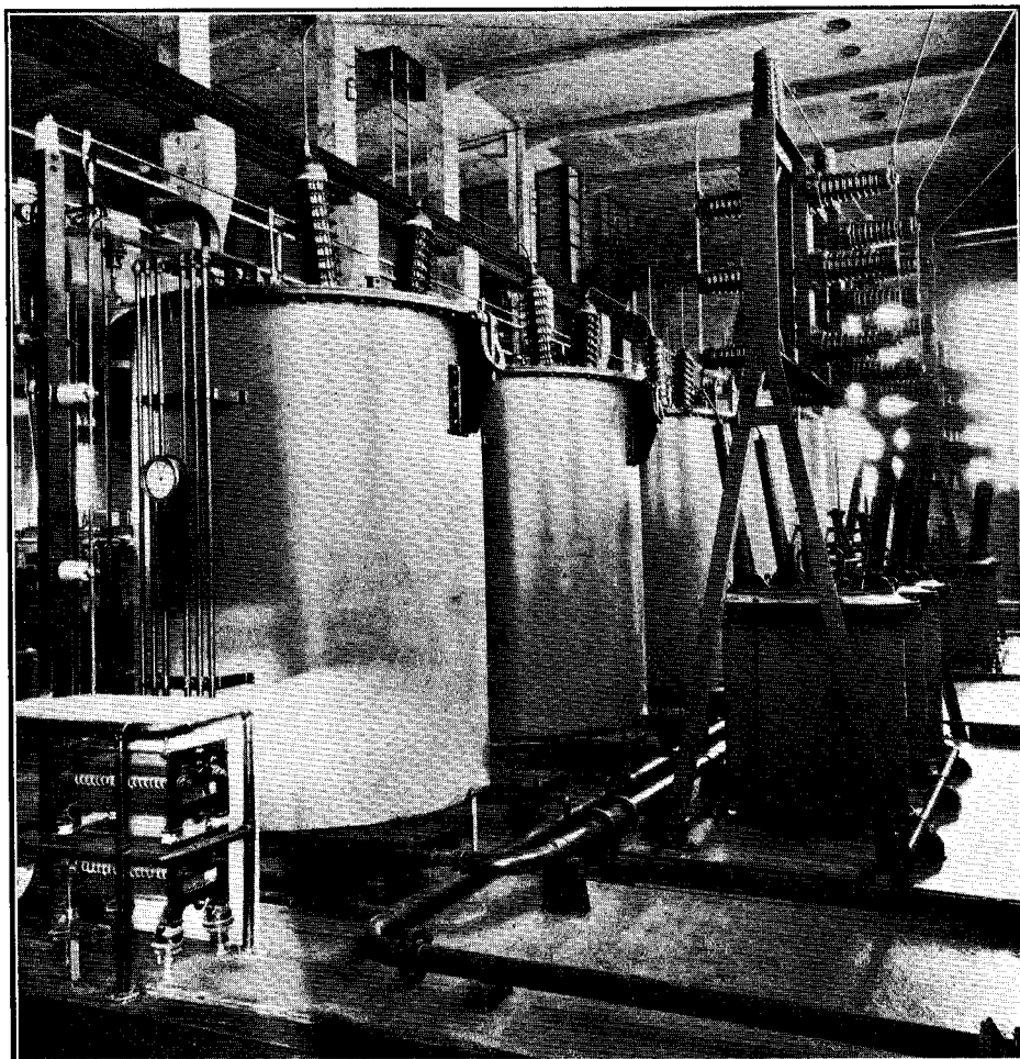
ADDINGTON SUBSTATION. 66,000-volt transformers and switch-gear.
