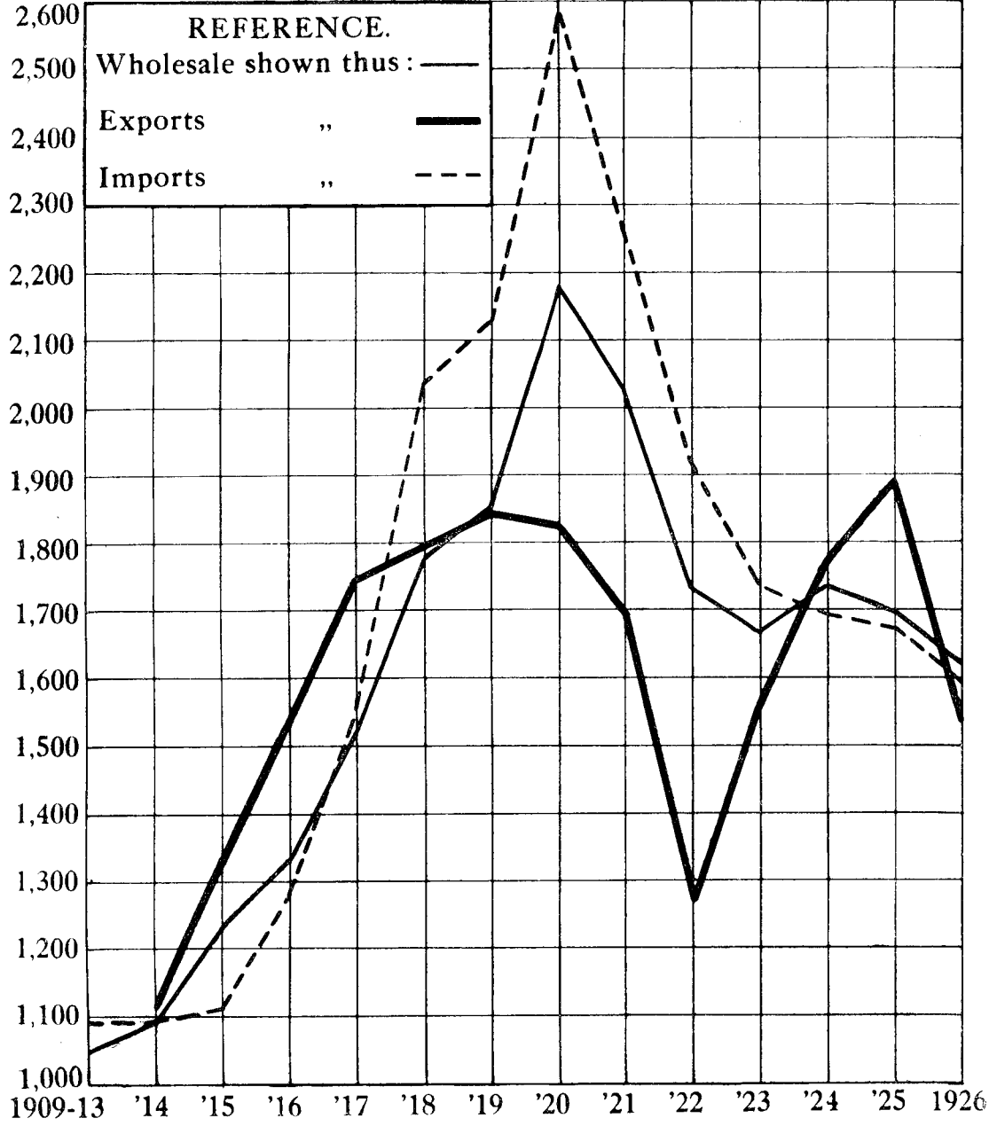
Index Numbers of Wholesale Prices, Export Prices, and Import Prices: Base 1909-13 = 1,000. Year-book, 1928, p. 781
