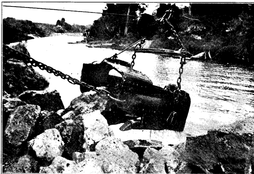
Drag-line Bucket in Rock, No. 1 Bar.
