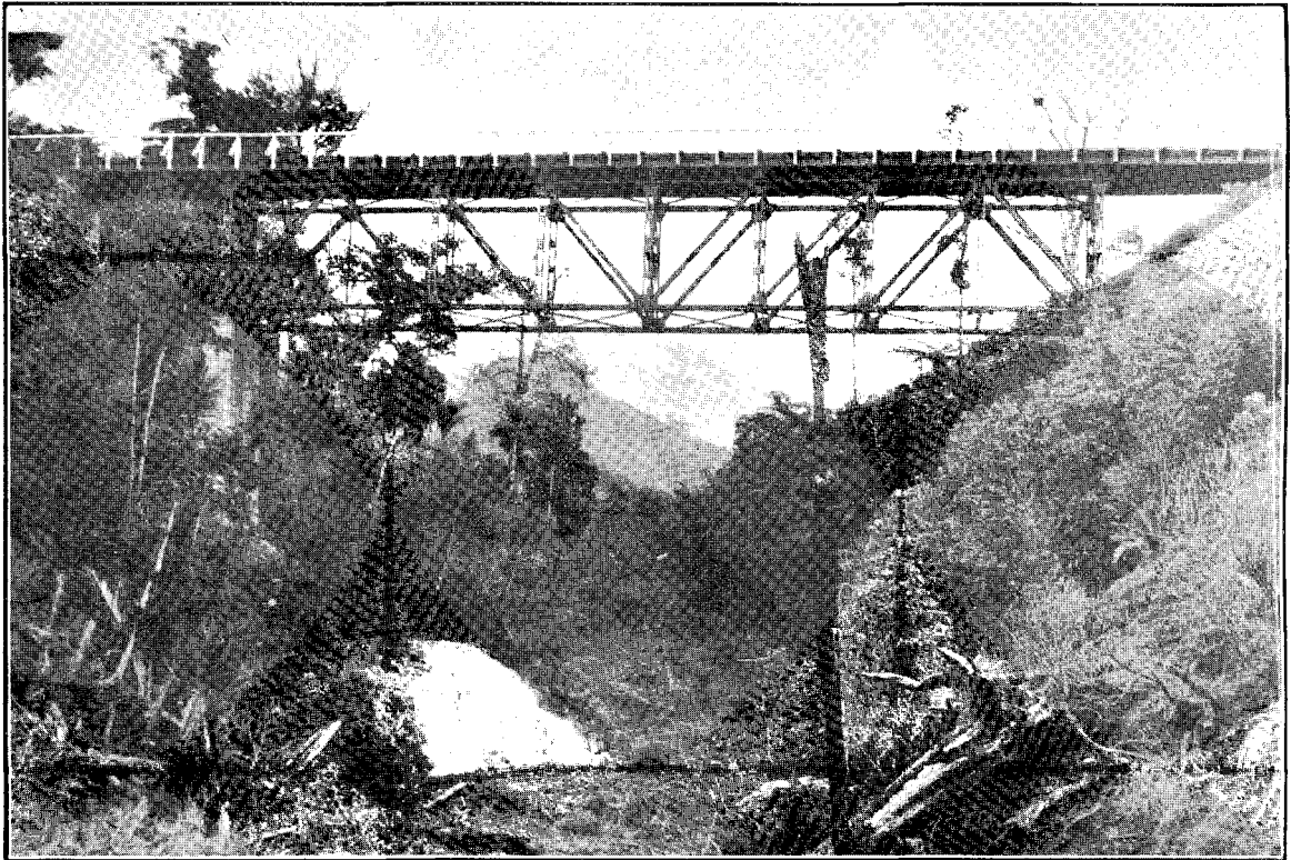
SIDE VIEW OF 120 FT. TRUSS. MANGATIPA RIVER BRIDGE.—KIRIKOPUNI-PARAKAO ROAD.
