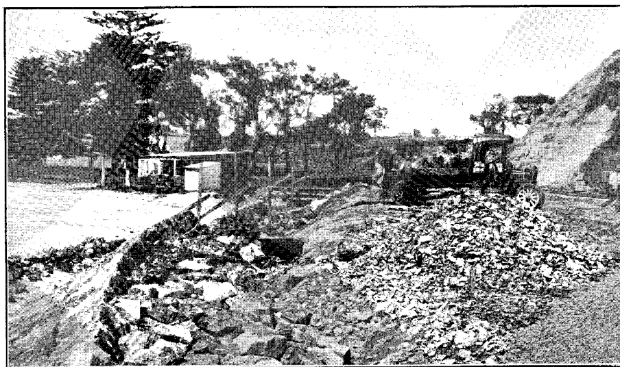
MISSION BAY EXTENSION : STONE PROTECTION AT 4 M. 0 CH.
