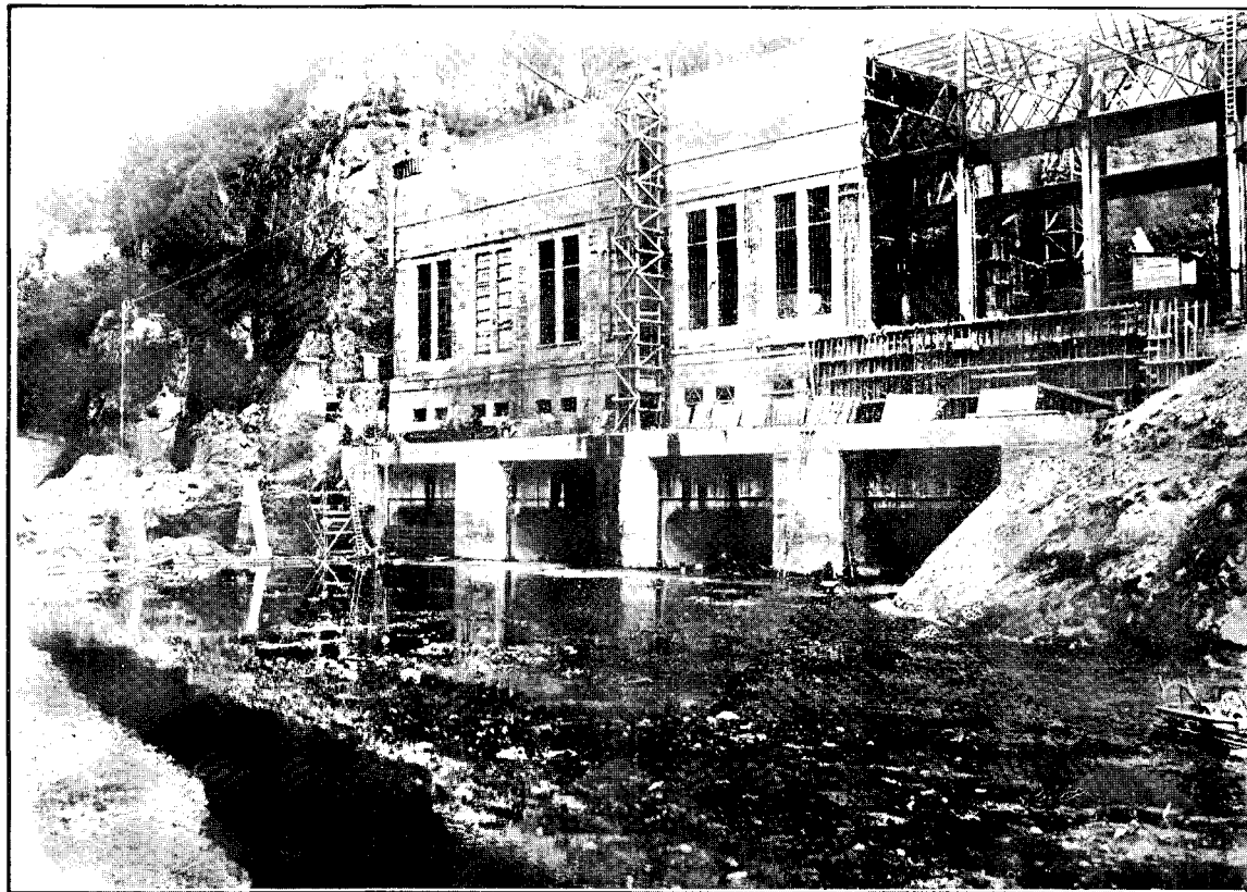
POWER-HOUSE DURING ERECTION, SHOWING TAIL-RACE AND DRAUGHT-TUBES.
