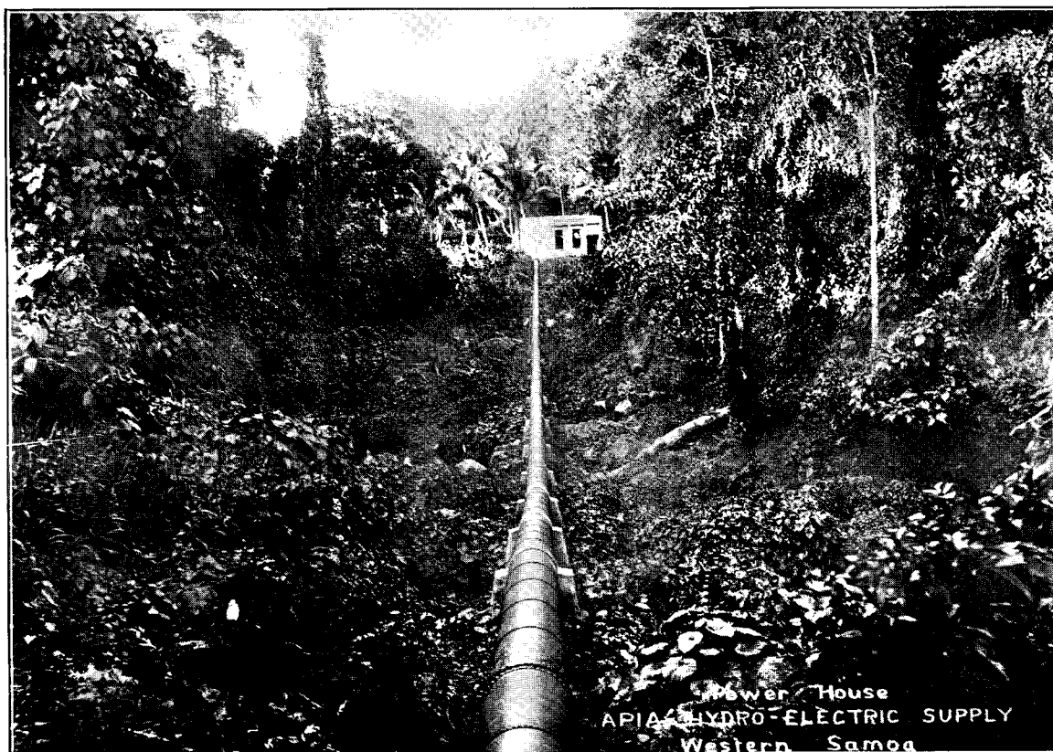
POWER-HOUSE AND PIPE-LINE. APIA POWER DEVELOPMENT.
