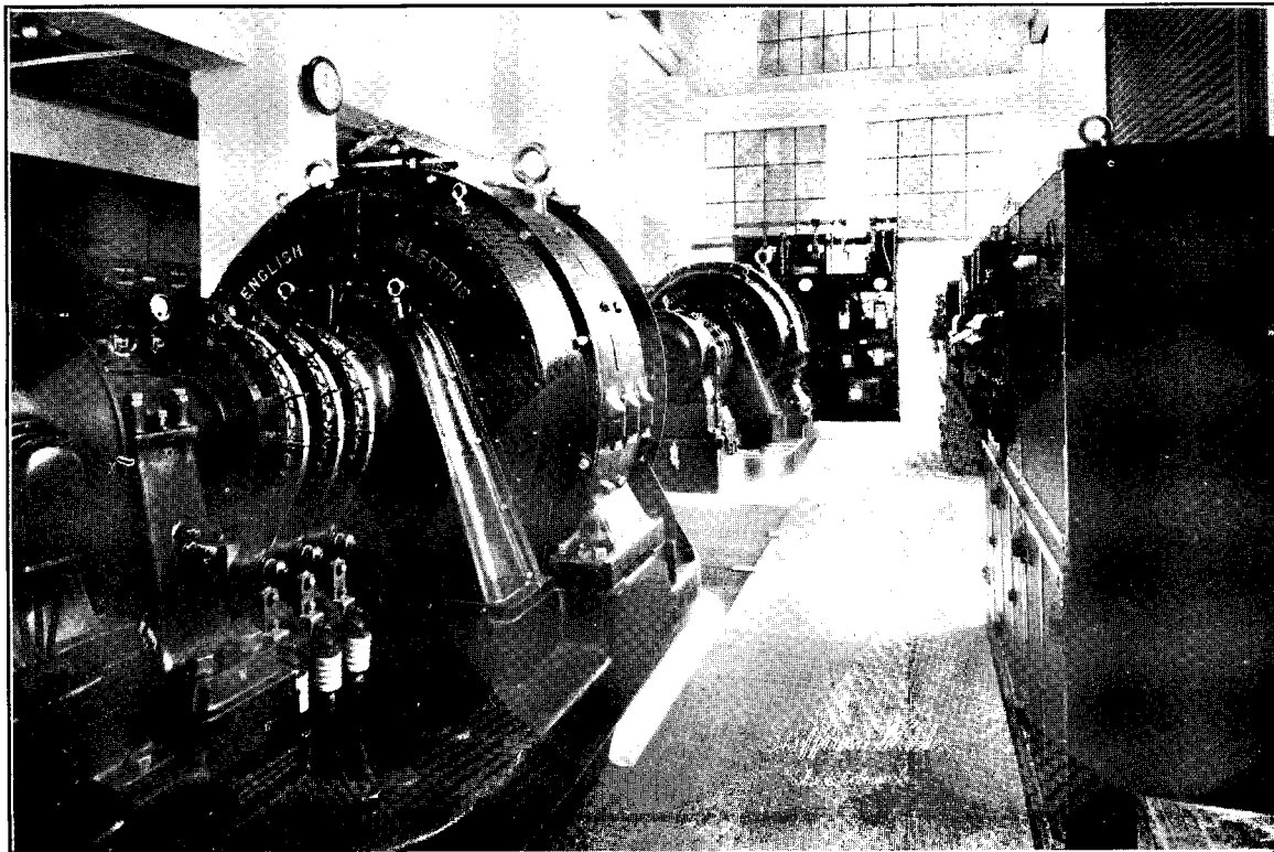
WOOLSTON SUBSTATION : 1,350 kw. 1,500-volt. ROTARY CONVERTOR. LYTTELTON-CHRISTCHURCH RAILWAY ELECTRIFICATION.
