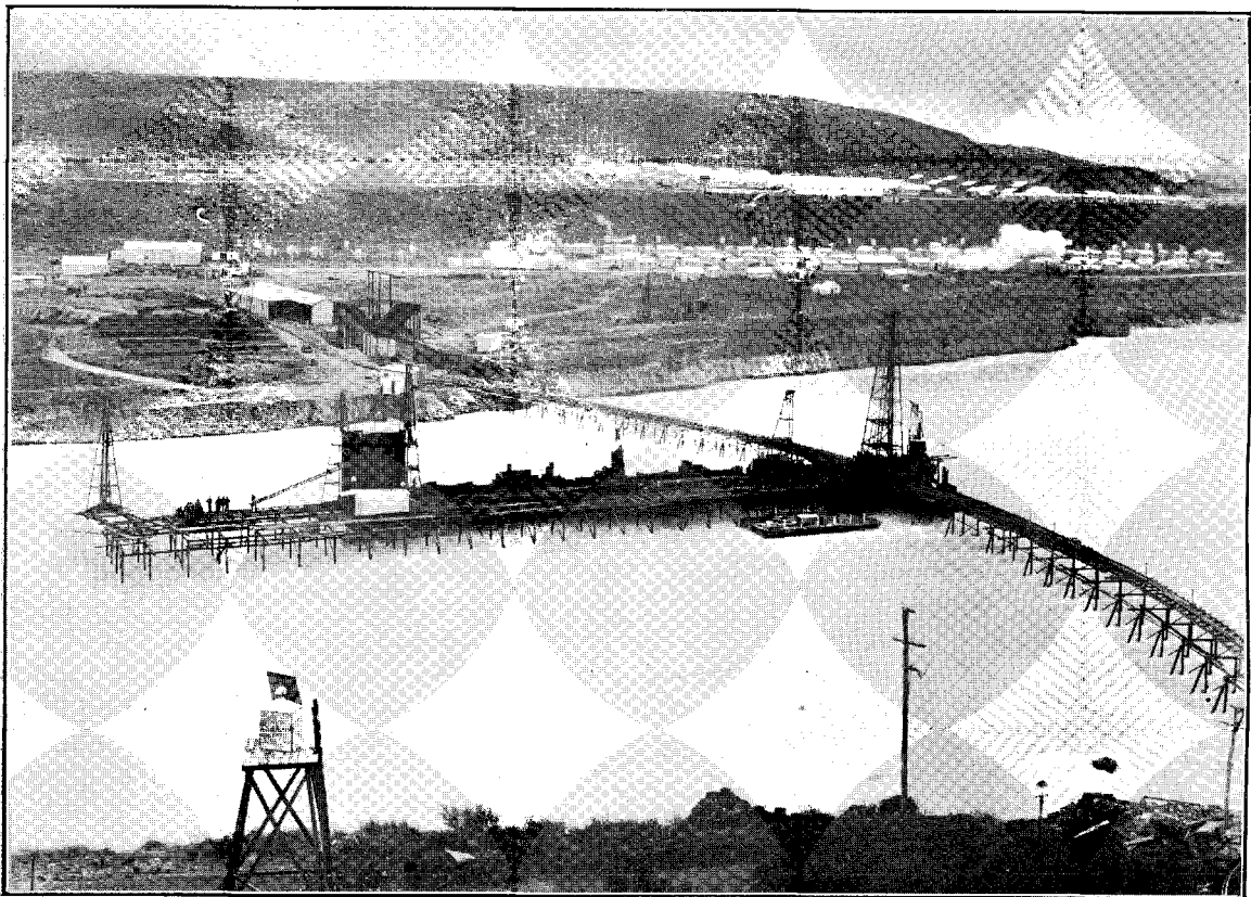
WAITAKI DAM: DRIVING SHEET PILING.
