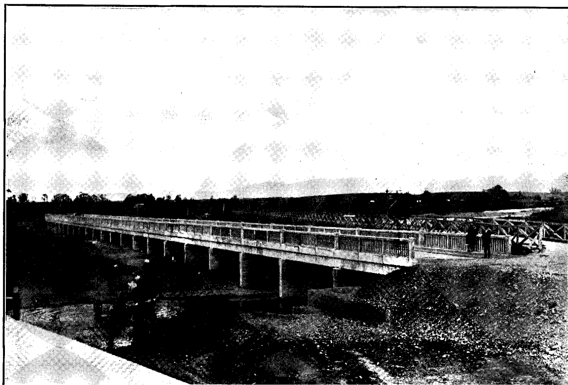
PAREORA RIVER BRIDGE. Twenty-two 30 ft. reinforced-concrete spans ; 18 ft. roadway. CHRISTCHURCH-DUNEDIN MAIN HIGHWAY.
