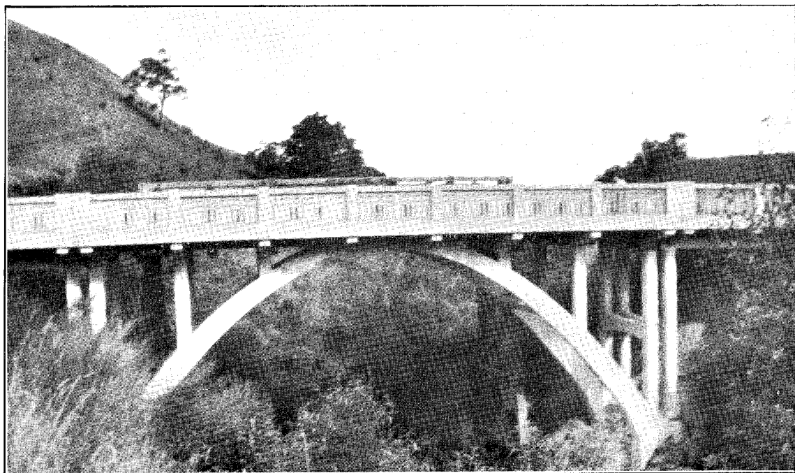
TE KURA BRIDGE.—REINFORCED CONCRETE ARCH. GISBORNE—WAIROA, VIA HANGAROA, MAIN HIGHWAY.
