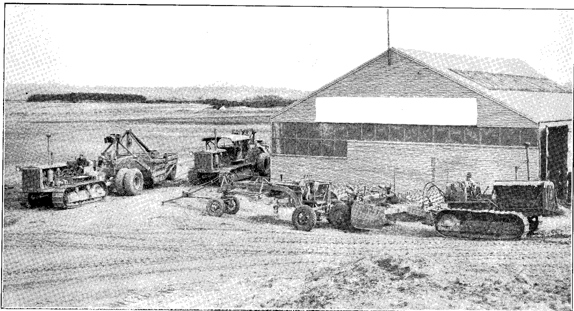
TYPICAL PLANT USED IN CONSTRUCTION. NELSON AERODROME.
