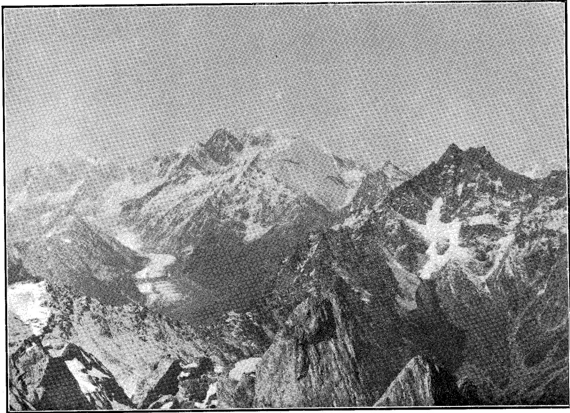
FIG. 7.—LOOKING INTO HEAD OF COOK RIVER FROM RYAN'S PEAK (6,890 FT.), SHOWING LA PEROUSE GLACIER.
