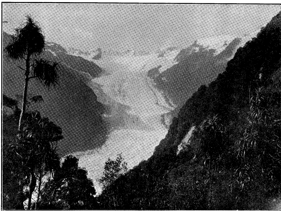
FIG. 10.—FRANZ JOSEPH GLACIER FROM 2,500 FT. ABOVE THE ICE (1893).
