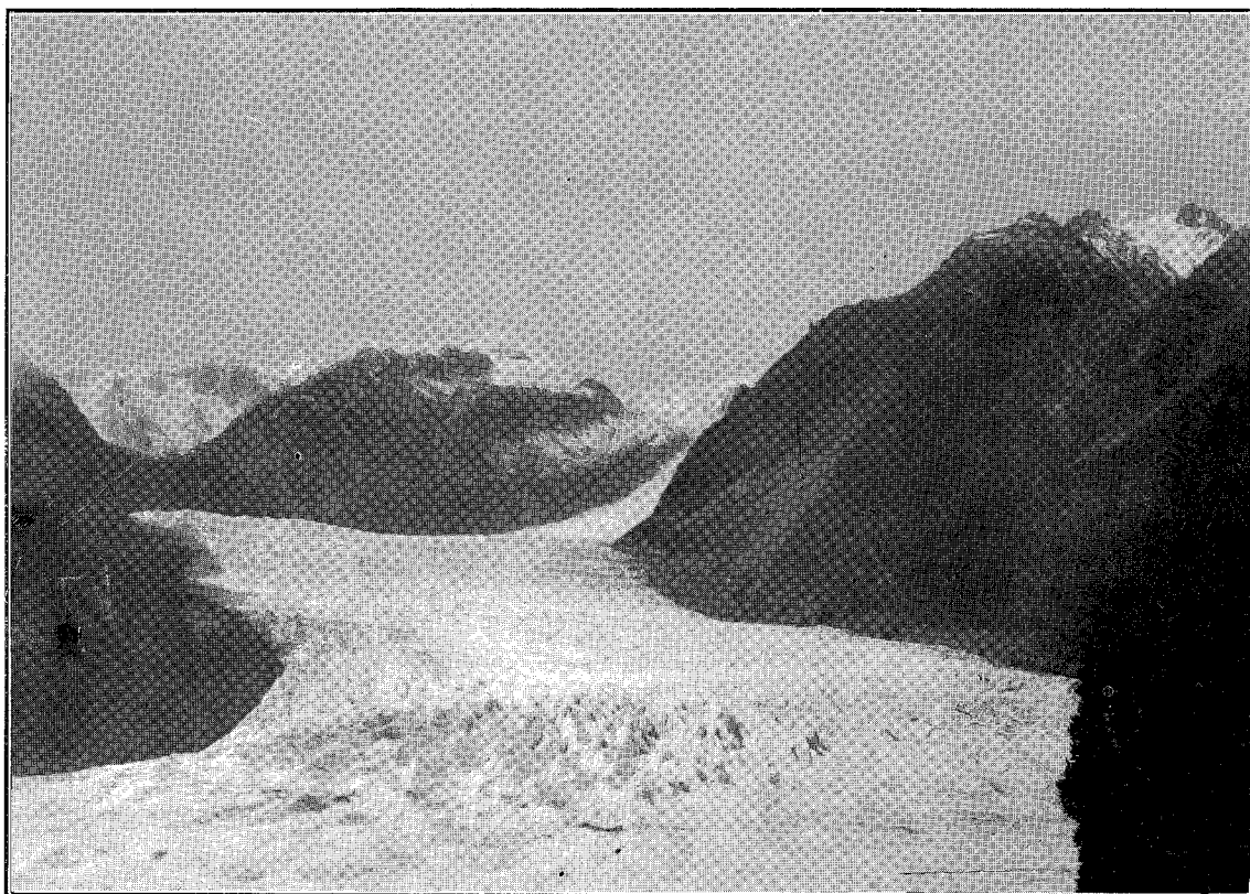
FIG. 9.—FOX GLACIER FROM CONE ROCK (1894).
