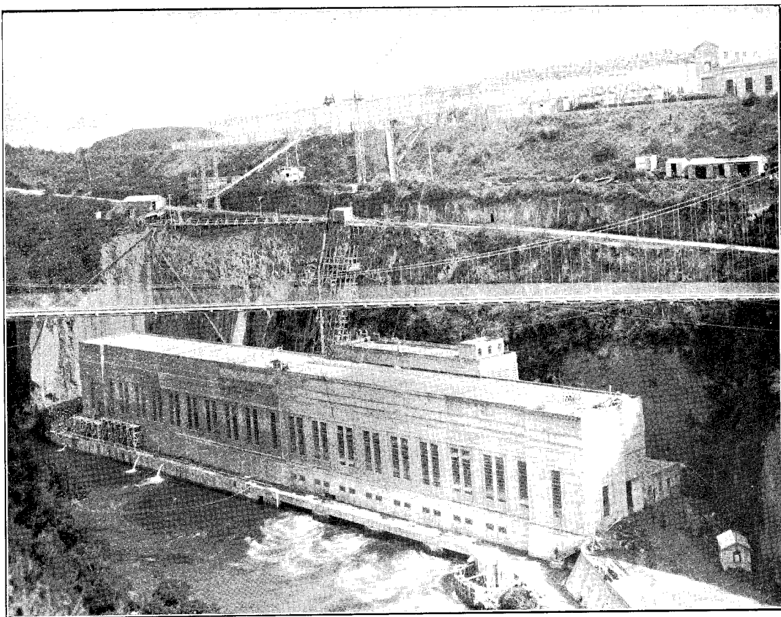
EXTENSION OF POWER-HOUSE AT ARAPUNI. NORTH ISLAND ELECTRIC-POWER SYSTEM.
