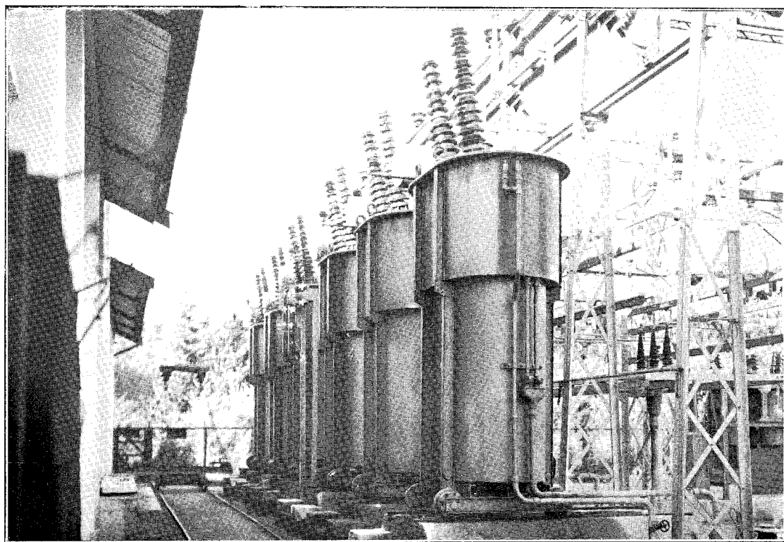
66 kV. TRANSFORMER BANK, MONOWAI. SOUTHLAND ELECTRIC-SUPPLY SYSTEM.
