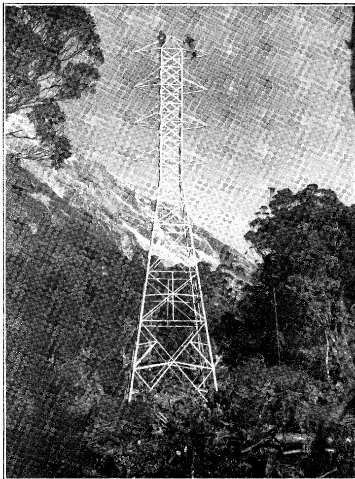
FIRST TOWER ON OTIRA — ARTHURS PASS SECTION OF 66 kV. LINE CONNECTING CANTERBURY WITH WESTLAND.
