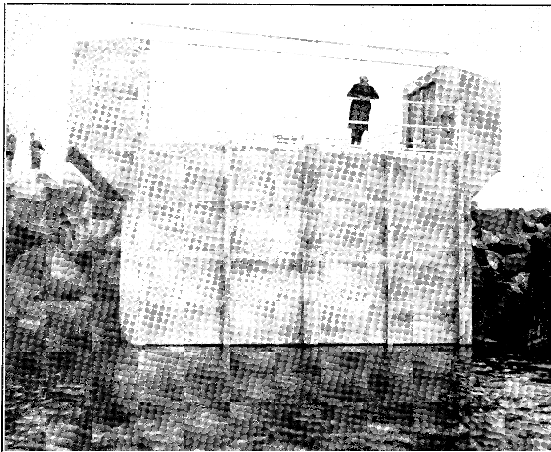
INTAKE STRUCTURE. LEVELS PLAIN IRRIGATION SCHEME.
