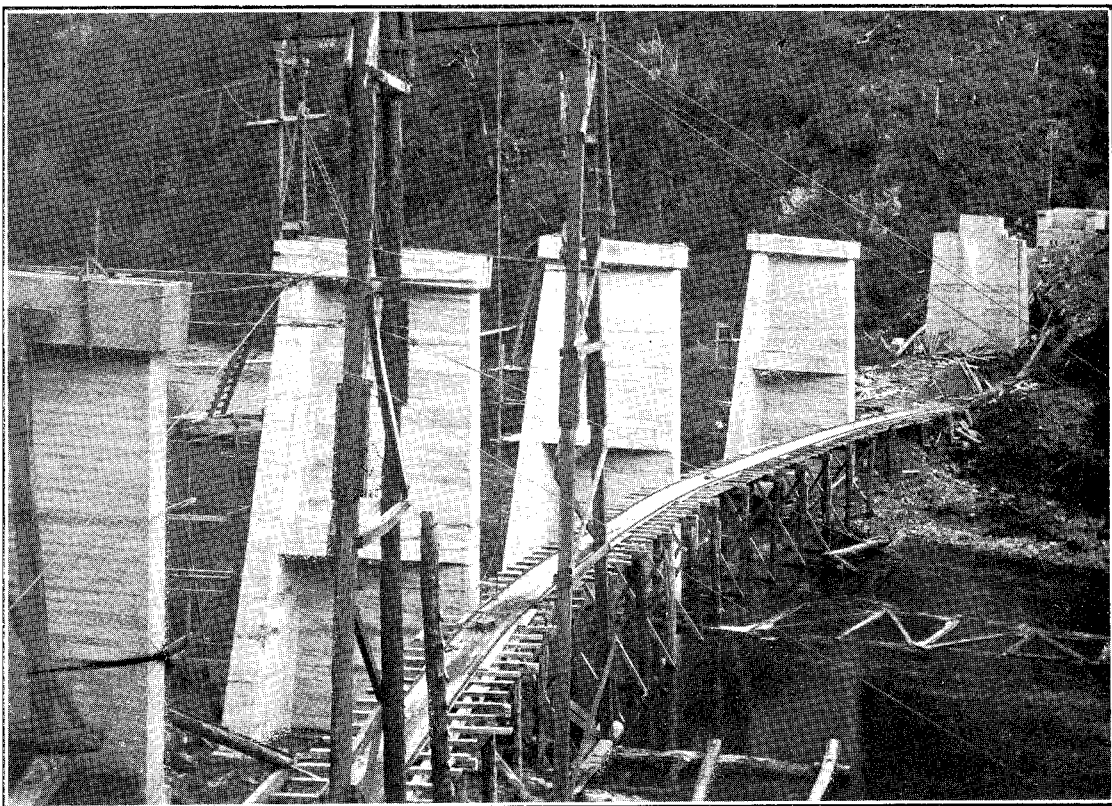
PIERS AND ABUTMENTS; AND GANTRY BEING ERECTED FOR PLACING GIRDERS IN POSITION. CASCADE CREEK BRIDGE, WESTPORT-INANGAHUA RAILWAY.
