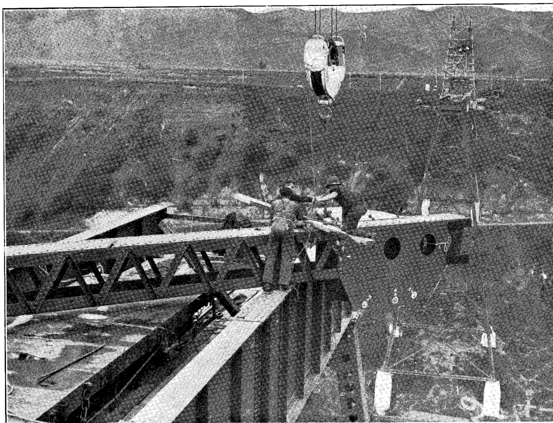
SECTION OF MAIN TOWER-LEG BEING SLUNG FOR LOWERING.
