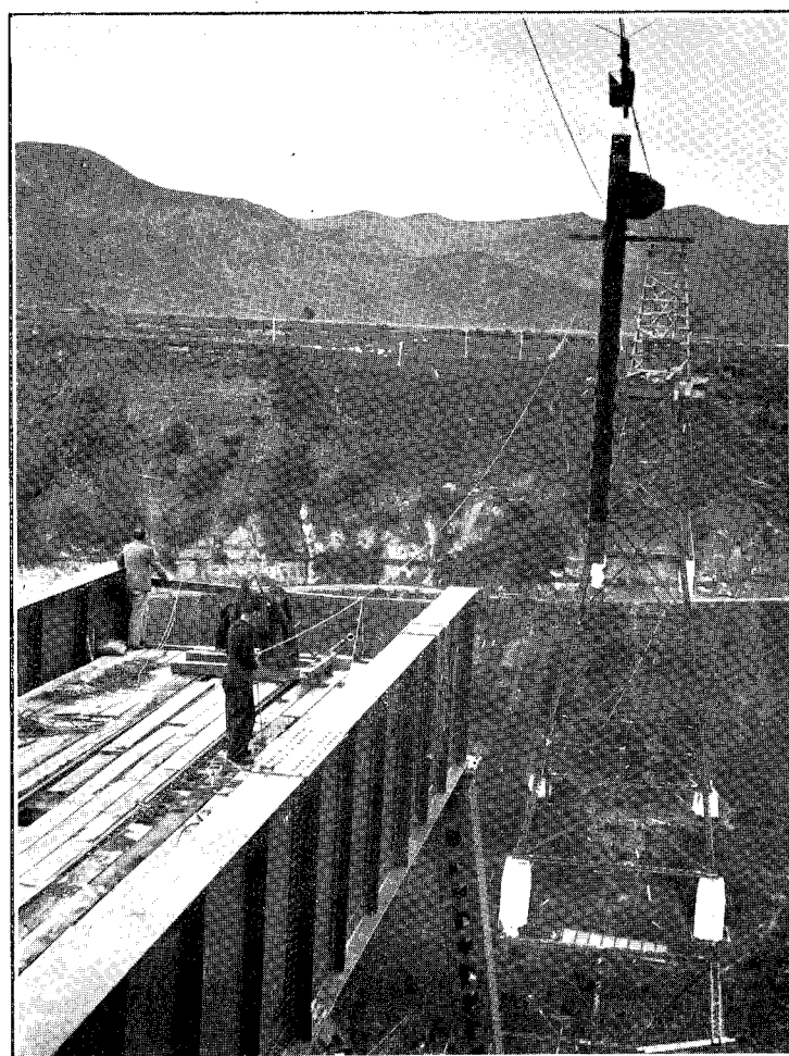
SECTION OF MAIN TOWER-LEG BEING LOWERED TO POSITION.
