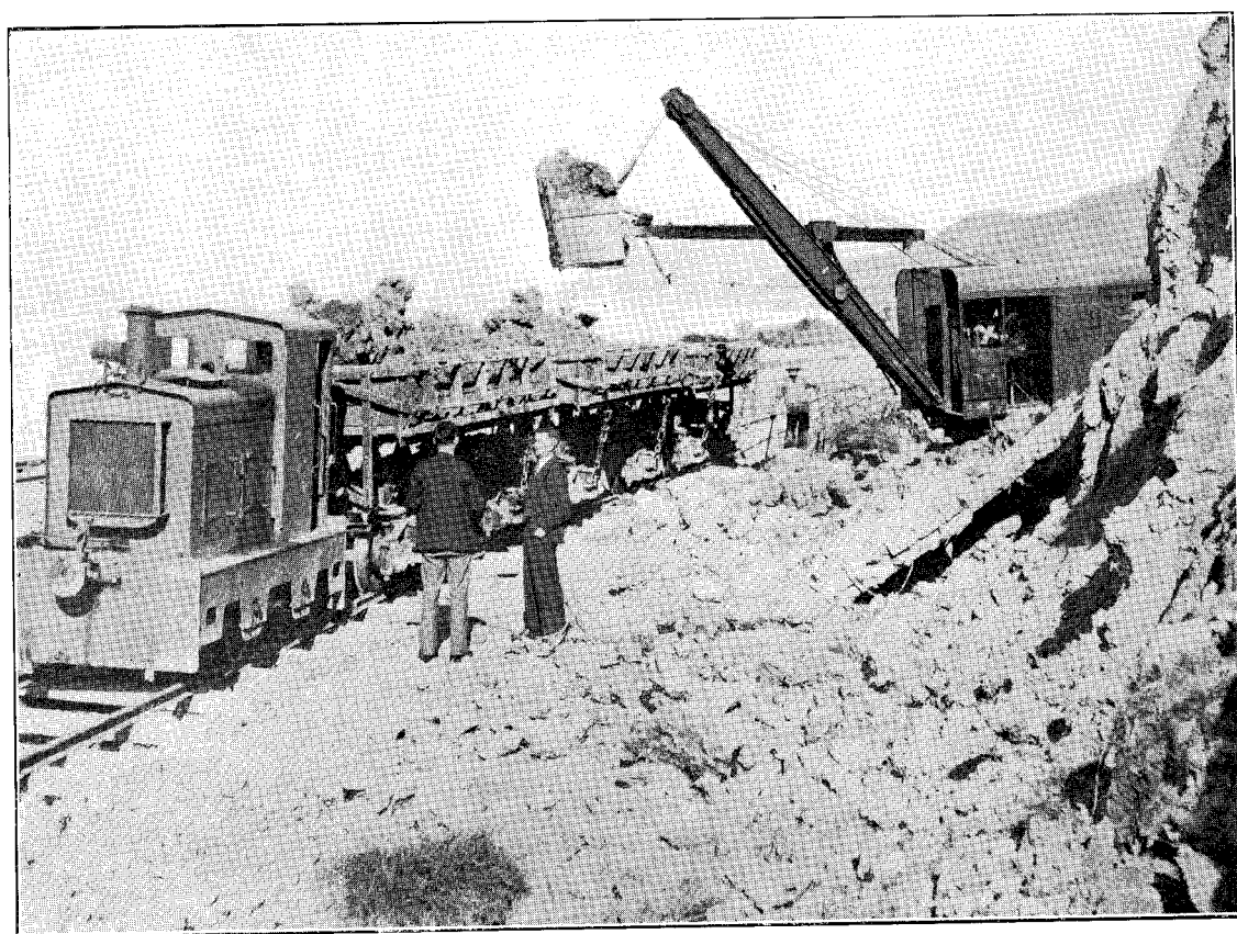
PLANT IN OPERATION REMOVING SLIP MATERIAL. SOUTH ISLAND MAIN TRUNK RAILWAY.
