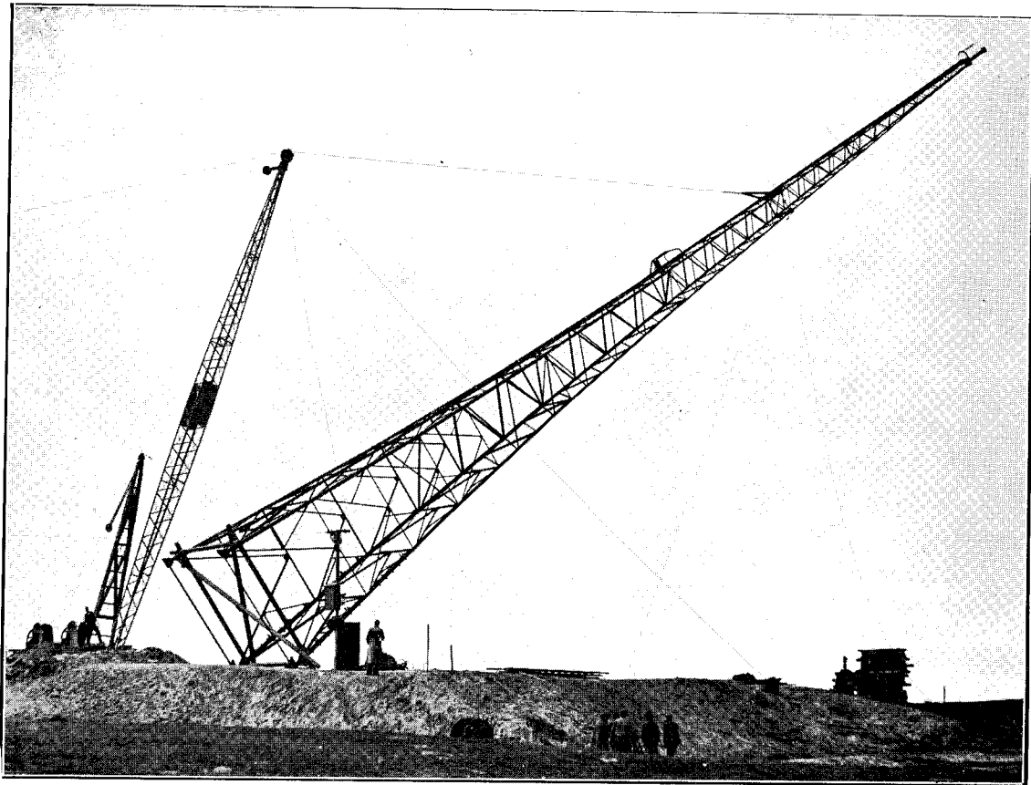
MAST BEING RAISED.
