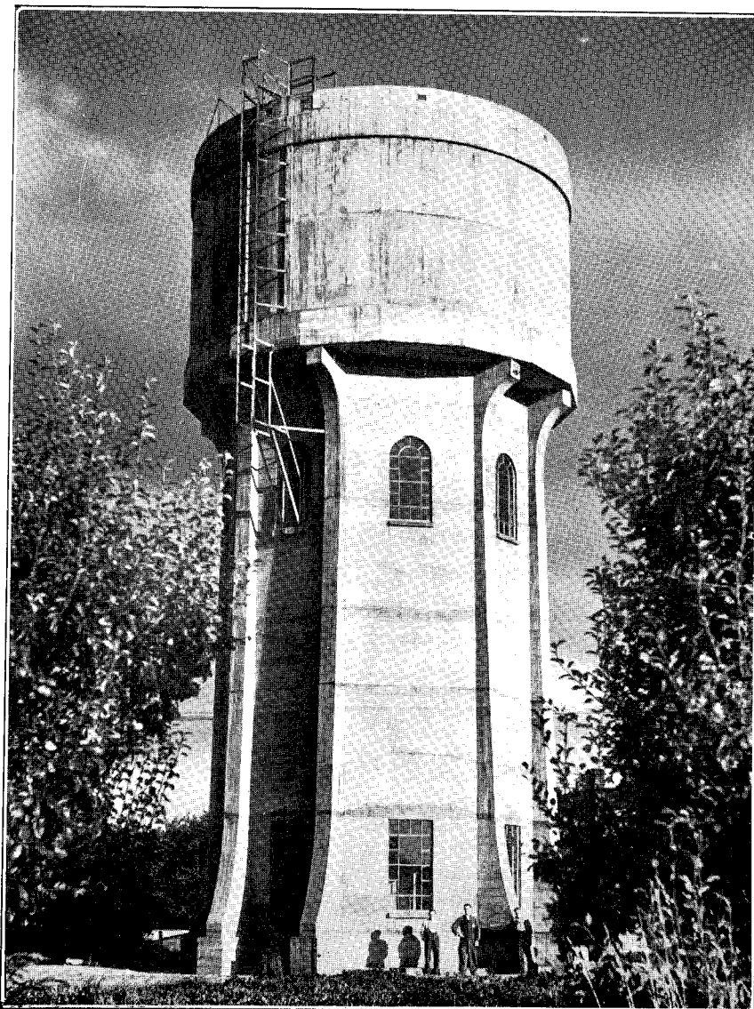
ELEVATED TANK OF REINFORCED CONCRETE 100,000 GALLONS CAPACITY. SUNNYSIDE MENTAL HOSPITAL.
