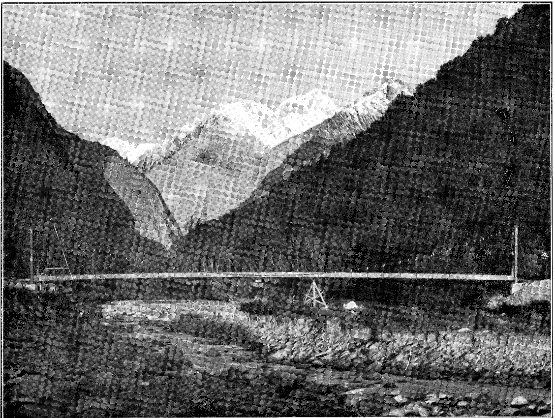
FOX RIVER SUSPENSION BRIDGE. MAIN SOUTH ROAD, WESTLAND.
