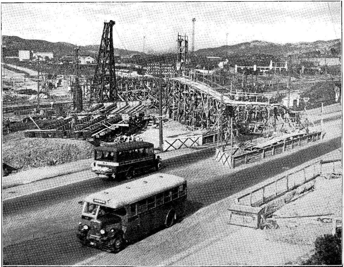
GENERAL VIEW, SHOWING PROGRESS OF CONSTRUCTION. THORNDON OVERBRIDGE, WELLINGTON CITY.
