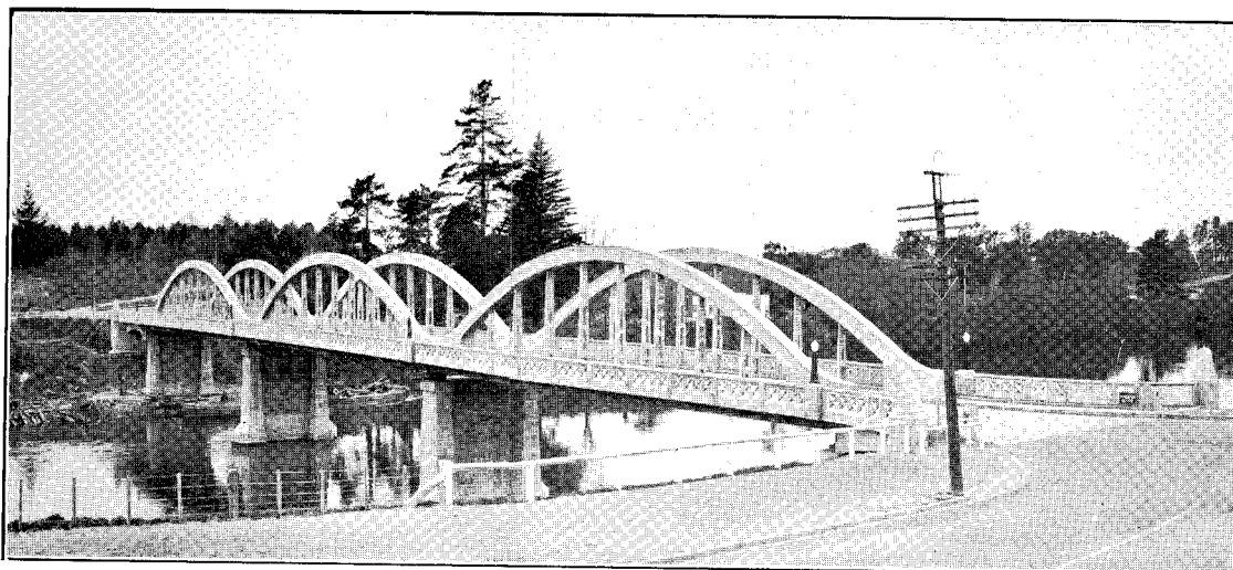
ROAD BRIDGE OVER WAIKATO RIVER, FAIRFIELD, HAMILTON. MAIN SPANS, 130 FT. BOWSTRING ARCHES IN REINFORCED CONCRETE.
