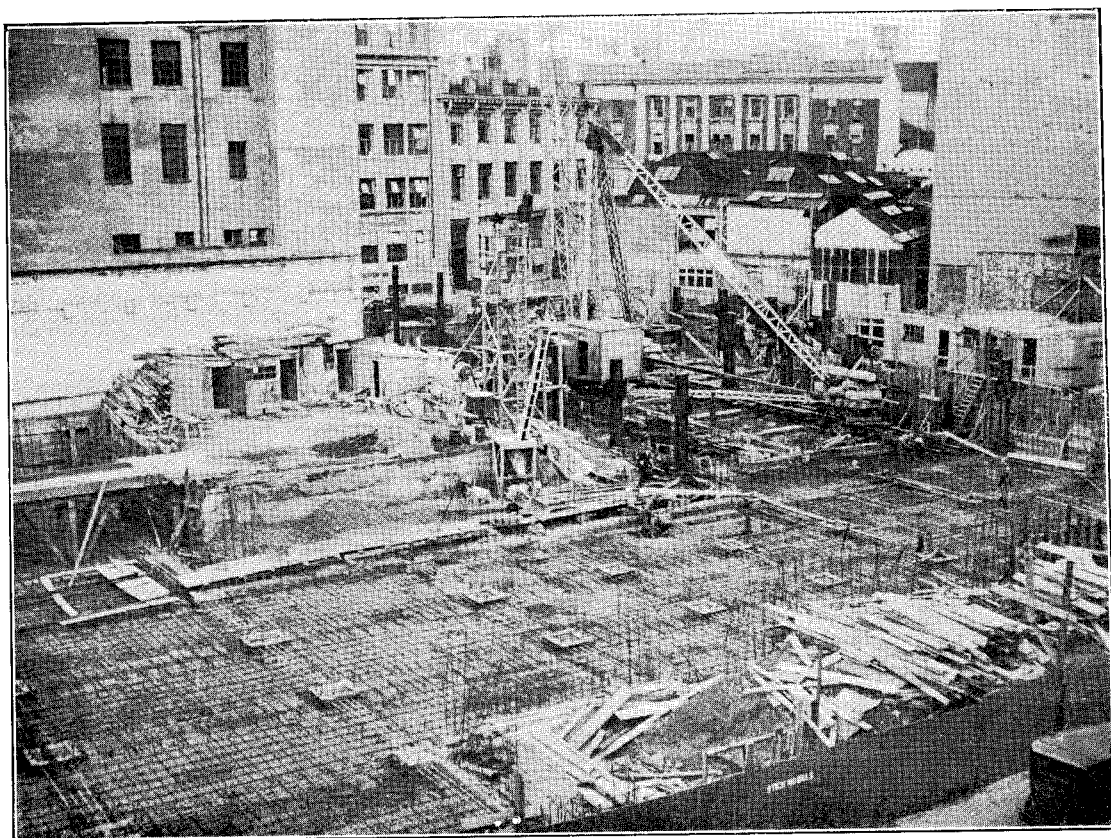
CONSTRUCTION OF FOUNDATION. NEW GOVERNMENT BUILDINGS, WELLINGTON.
