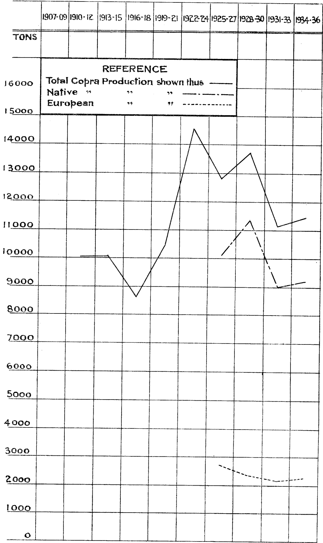
COPRA PRODUCTION, 1910-36.
