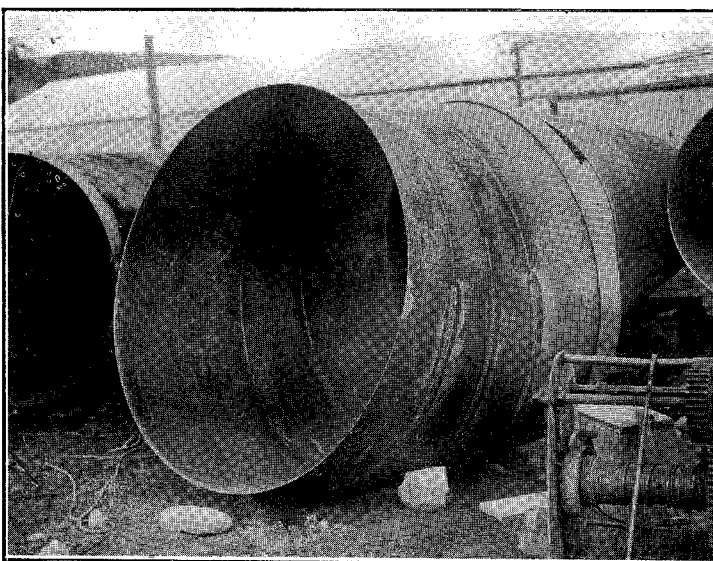
PIPE BEND, SHOWING WELDED CONSTRUCTION.
