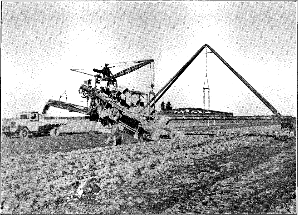
RUTH DREDGER, WITH CONVEYOR ATTACHMENT ON CONSTRUCTION OF WATER-RACE.
