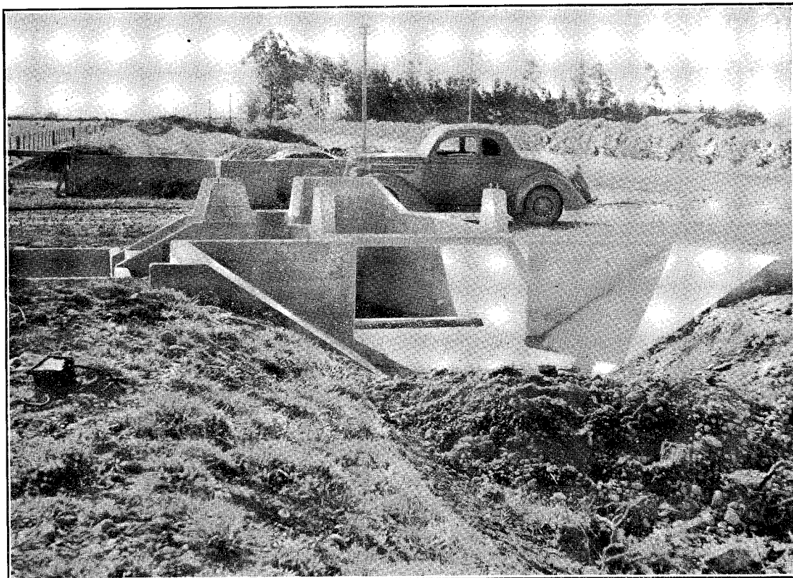
COMBINED ROAD-CROSSING SIPHON AND BIFURCATION-CONTROL STRUCTURE.
