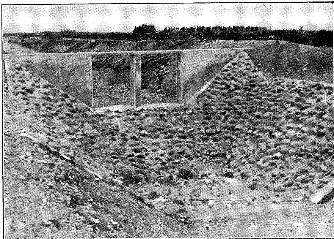
COBBLE-TYPE DROP.
